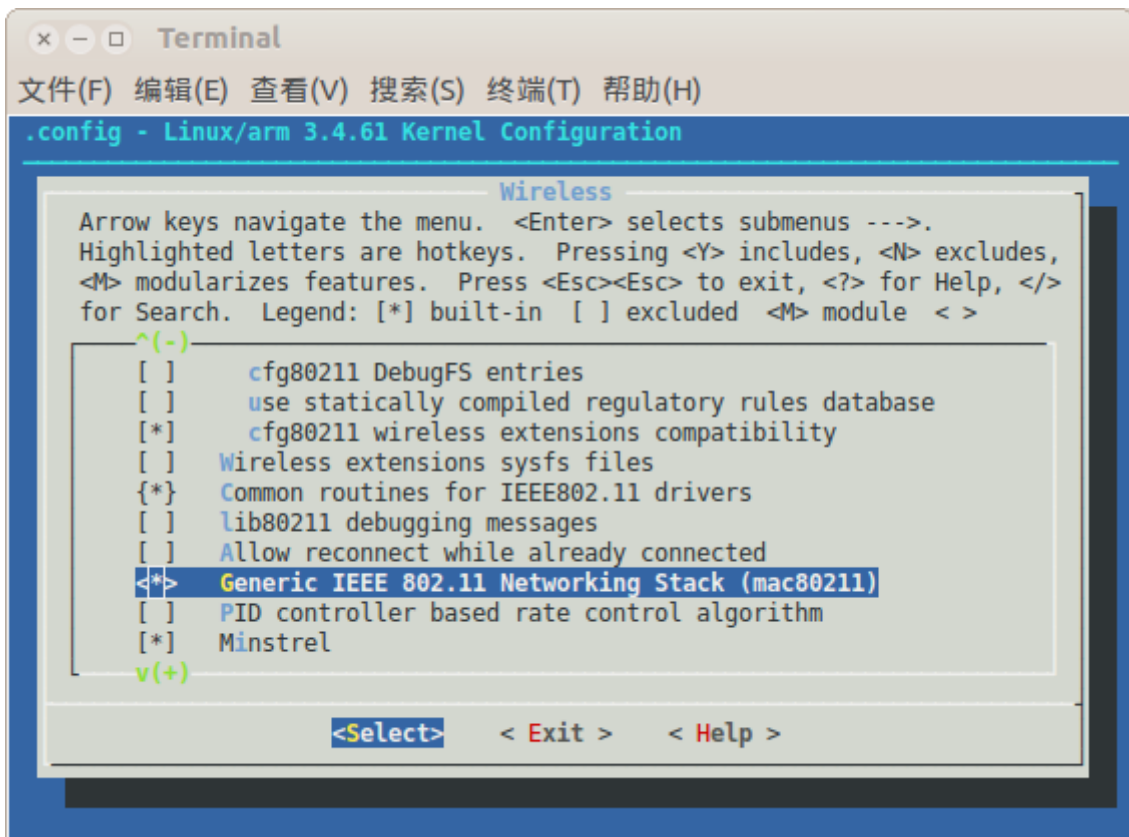
图 3: Networking support ---&gt; Wireless ---&gt; Generic IEEE 802.11 Networking Stack (mac80211)
